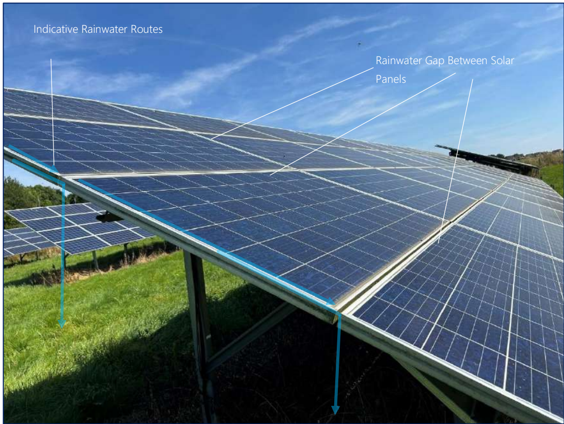
Plate 12-25 Rainwater gaps on PV array table
